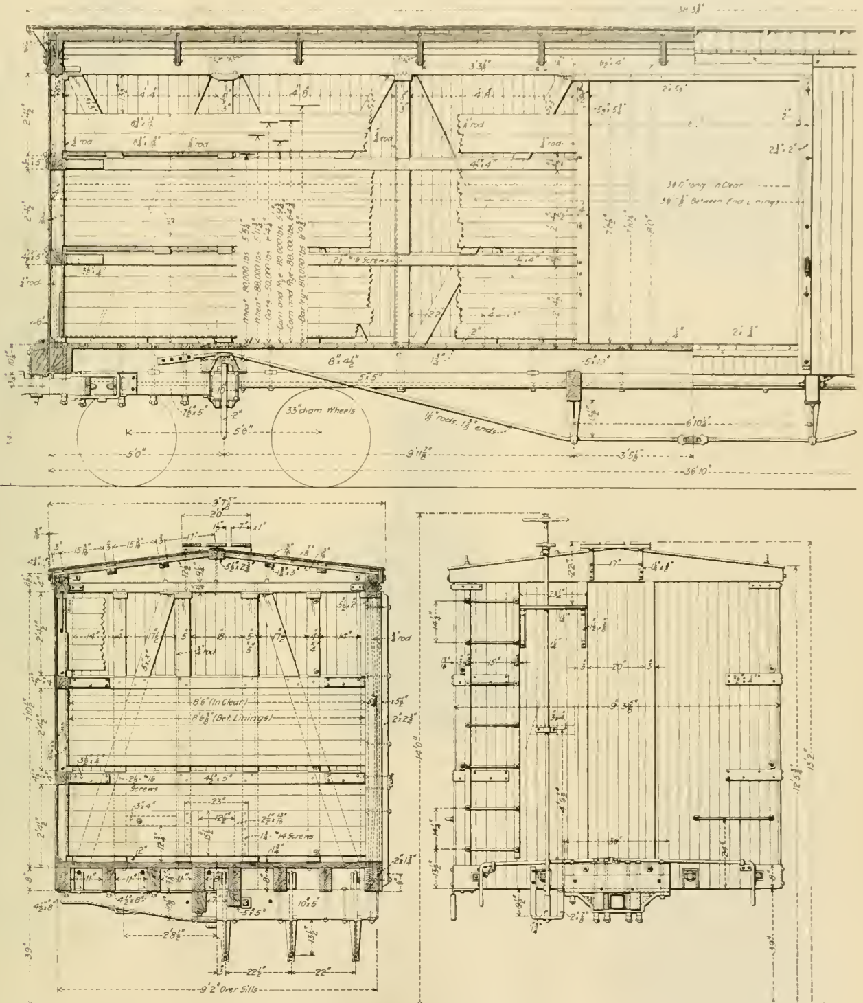
DETAILS OF NEW YORK CENTRAL BOX CAR.
